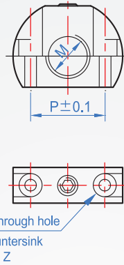
B : Vertical mounting
