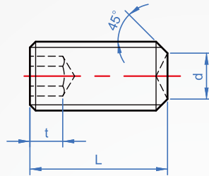
A Cup Point
