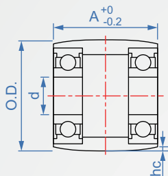
B type (barrel shape)
