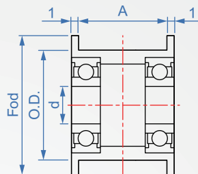
H type (flange type)
