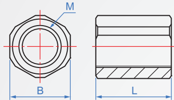
Straight : M8~M12
